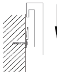
STEP 8 Press lightly to secure. Ensure the mirror is firmly mounted.
