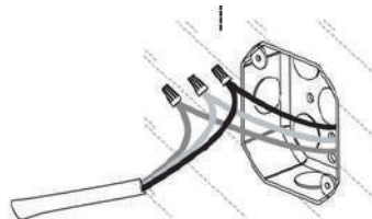
STEP 5 Connect the wires to the power supply: • Black wire → Live (L) • White wire → Neutral (N) • Green wire → Earth (E)
