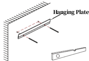
STEP 2 Mark the drill positions along the horizontal line. Use a spirit level to ensure they are level.
