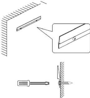
STEP 4 Fix the mounting bracket to the wall with screws.
