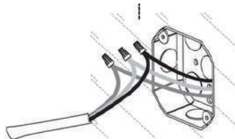
STEP 5 Connect the wires to the power supply: • Black wire → Live (L) • White wire → Neutral (N) • Green wire → Earth (E)
